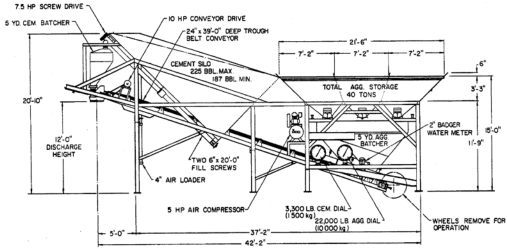
ROSS MODEL 110 RUSTLER BATCH PLANT 5 YARD BATCHING SYSTEM
